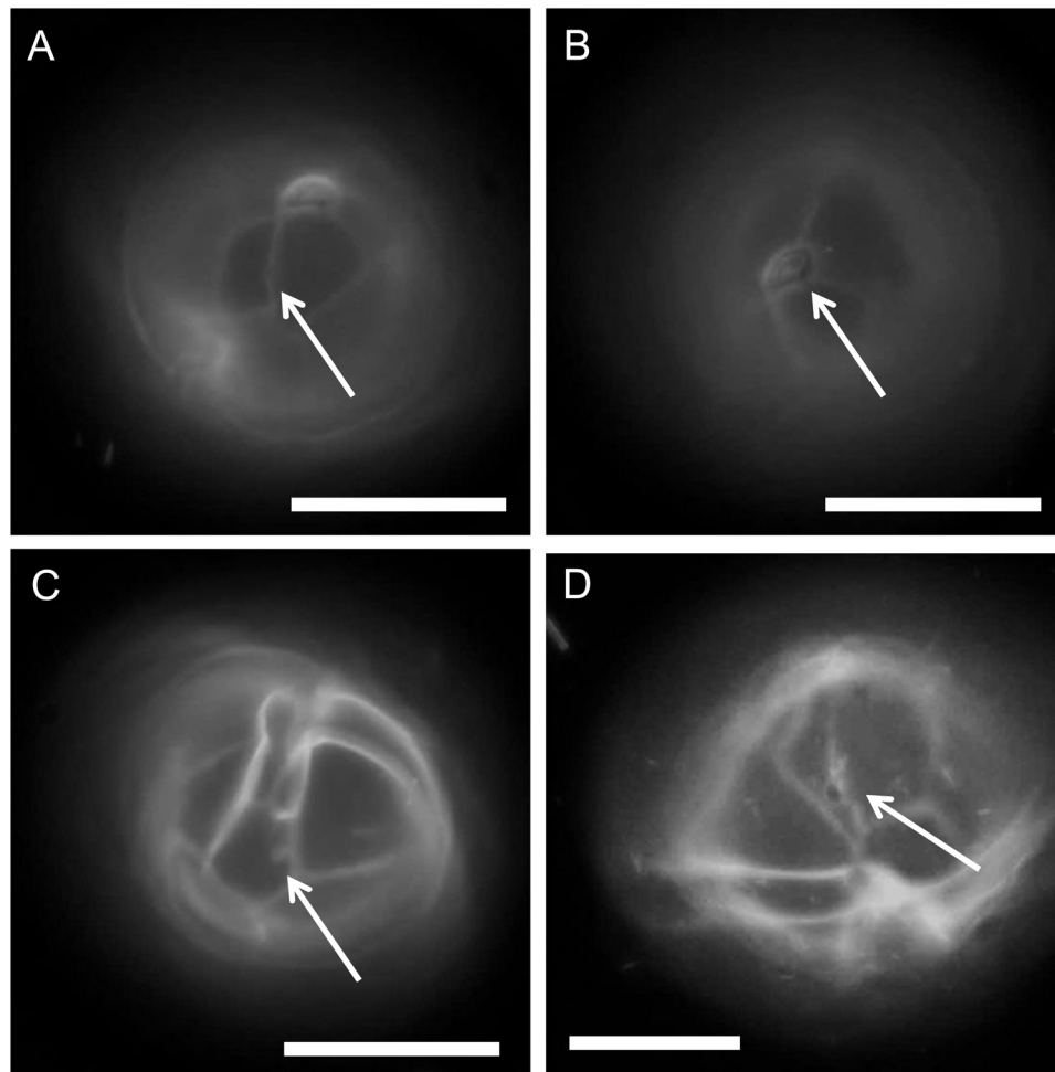
Fig. 2. Microphotographs of Alexandrium tamarens and A. ostenfeldii vegetative cells found at stations in the Chukchi Sea shelf. A–C show the same cells from different angles. White arrows indicate a ventral pore between the 1' and 4' plates (A), apical pore complex (B), sulcal plate (C), and a ventral pore between the 1' and 4' plates of A. ostenfeldii (D). Scale bars = 20 \mu m .
